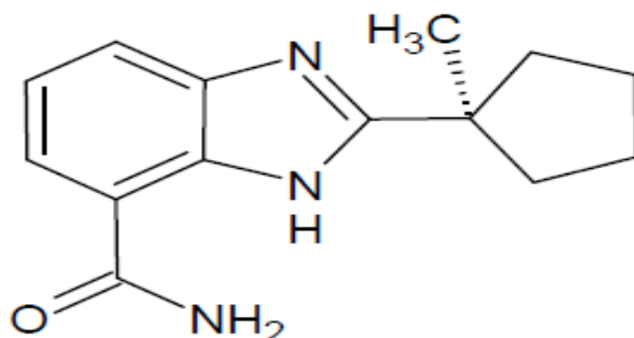
Figure 16: (2-((R)-2-methylpyrrolidine-2-yl)-1H-benzimidazole-4-carboxamide).
